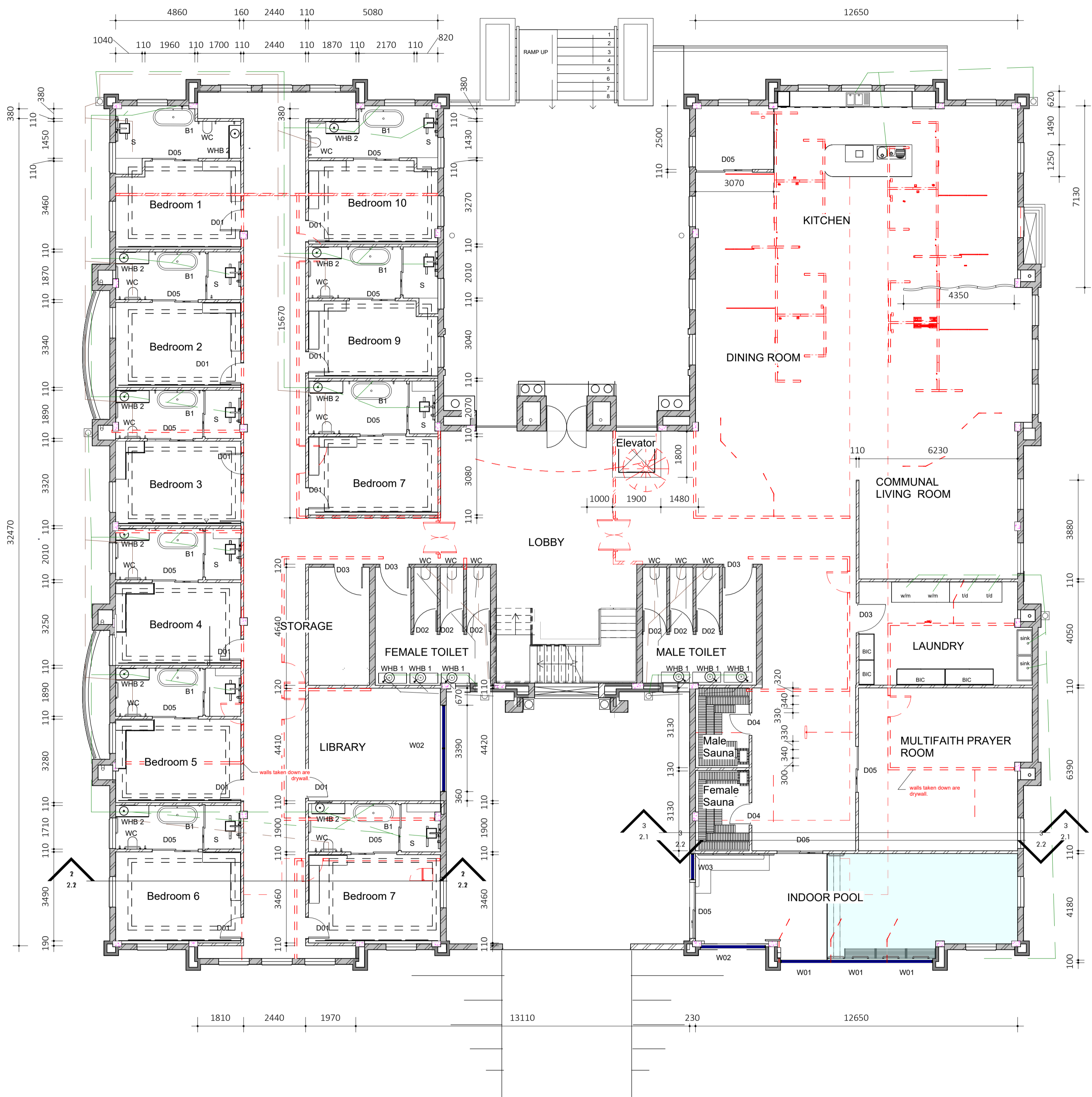
2.1 1.0 GF - Alterations Layout 1 : 100
