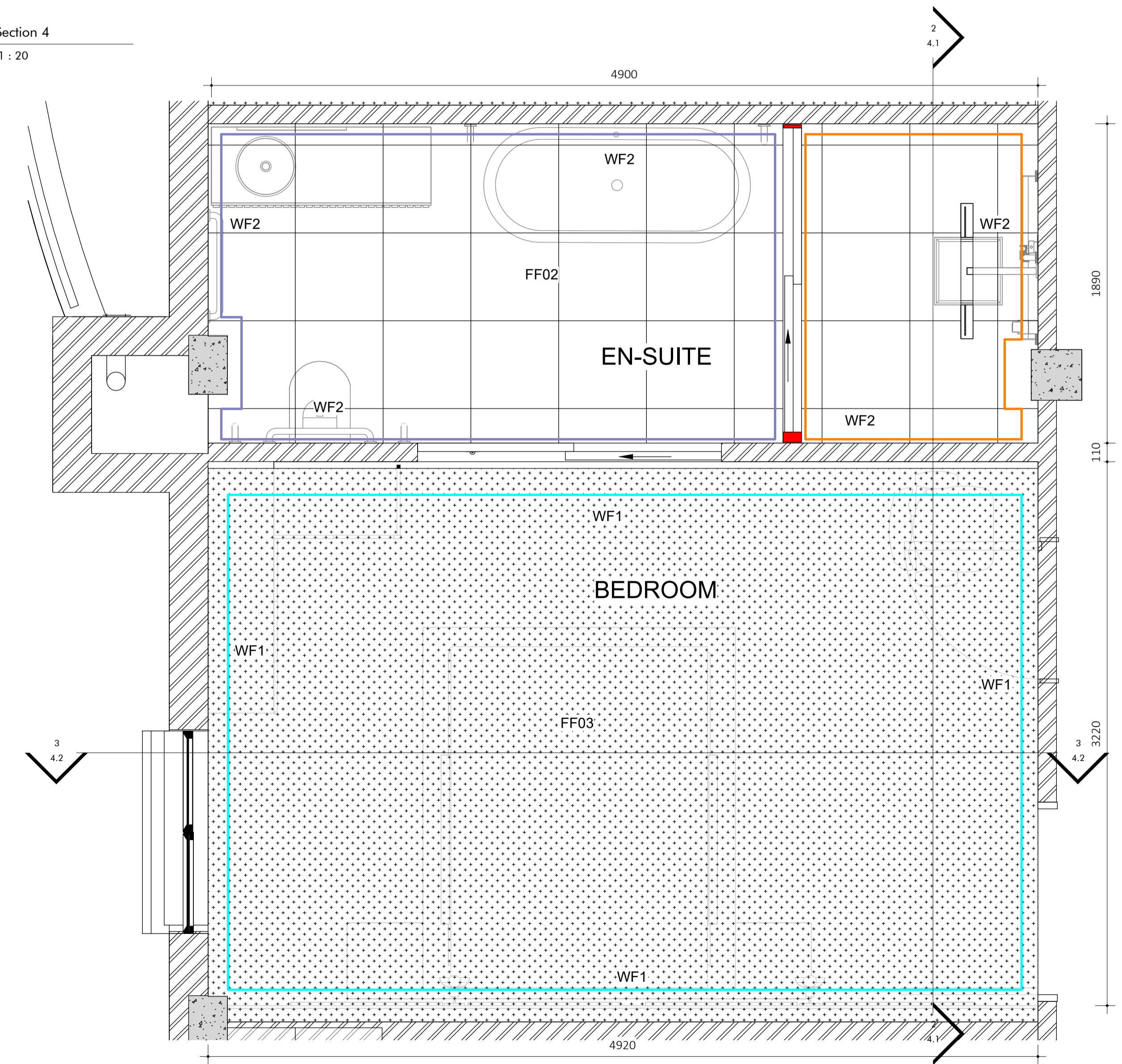
4.2 0. GF - Bedroom Floor + Wall Finishes Plan 1 : 20
